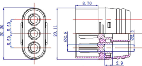
MR60 Male
