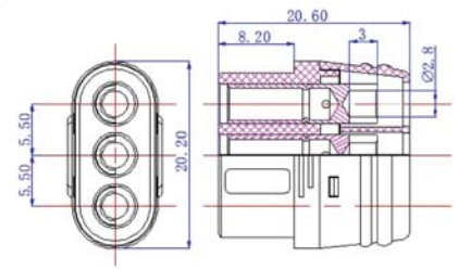
MR60 FEMALE
