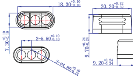
MR60 BACKSHELL
